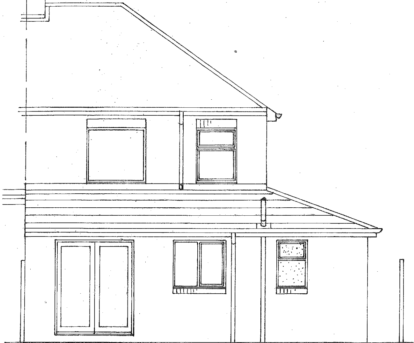
PROPOSED REAR 1:50
