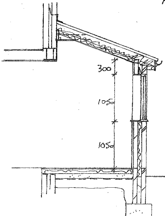
SECTION 1:50
